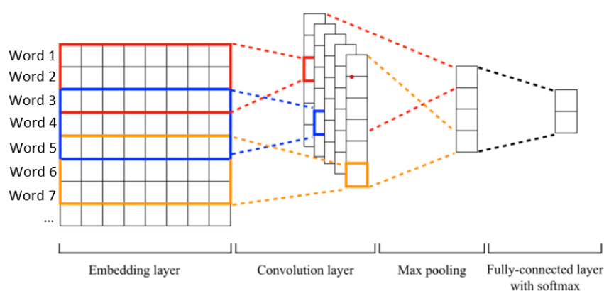
Figure 41 CNN model architecture for text processing.
