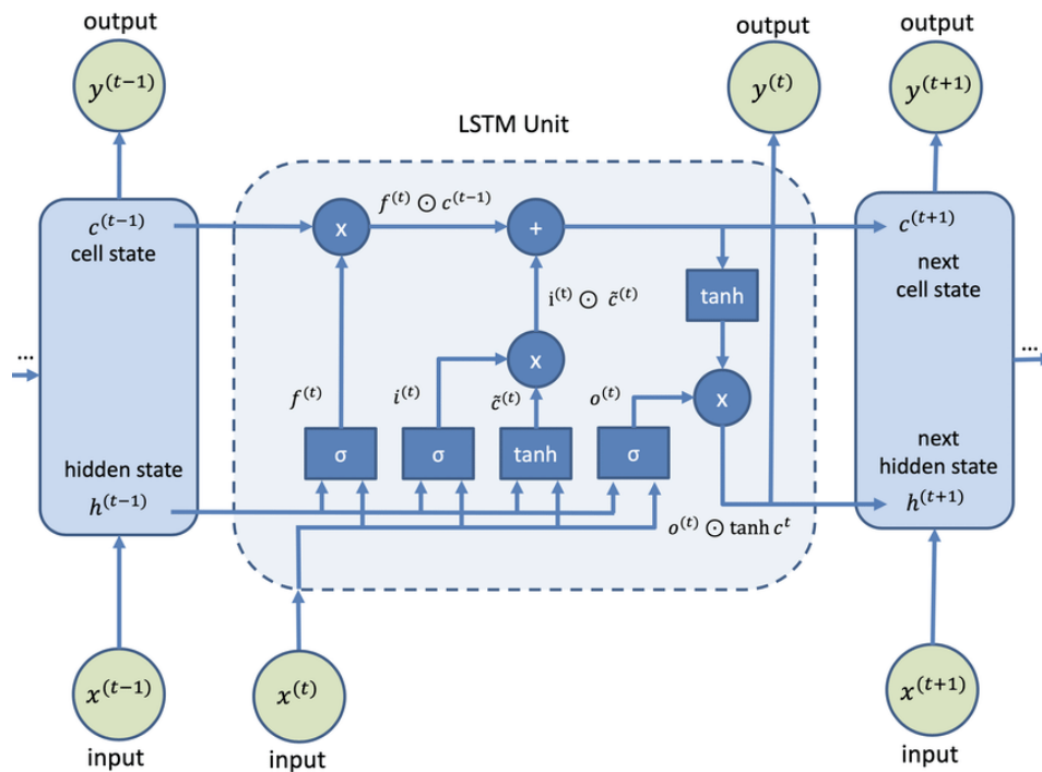
Figure 30 LSTM unit architecture.
