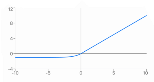
Figure 27 ELU activation function graph.
