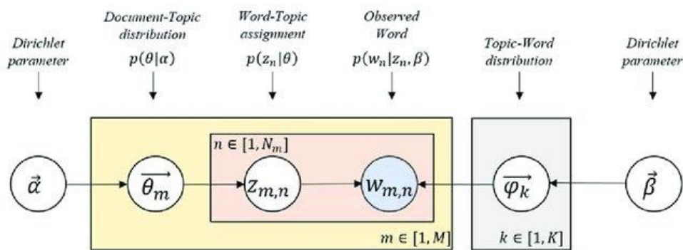
Figure 40 Architecture of LDA model.
