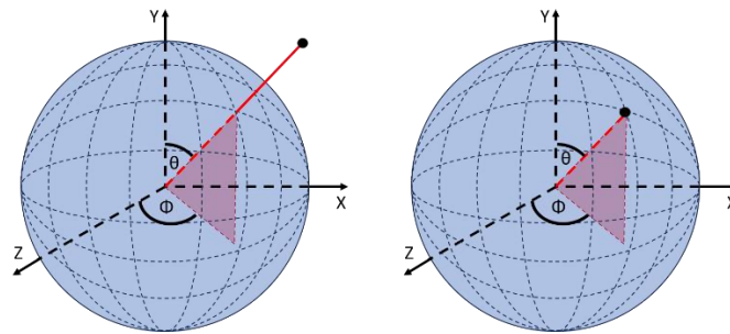
Figure 25 Word vector normalisation process. Each vector is adjusted such that its lies at some point on a 3D spherical plane of radius 1. As angles \theta and \Phi are conserved in the process, sentiment is largely unaffected and strategies for comparison using cosine similarity are still valid.
