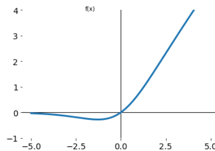
Figure 29 Swish activation function graph.
