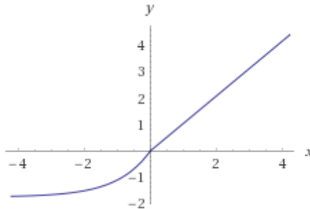
Figure 28 SELU activation function graph.
