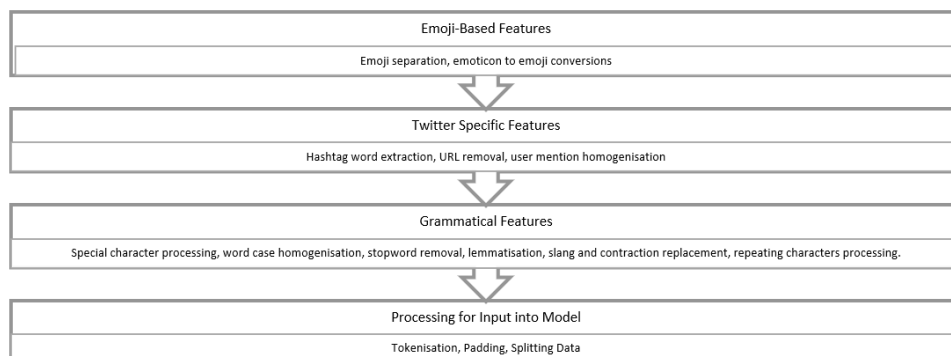
Figure 19 Data cleaning steps for neural network model training.
