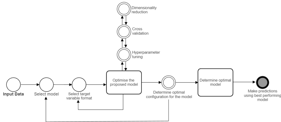
Figure 12 Process to select model for basic theory regression task.
