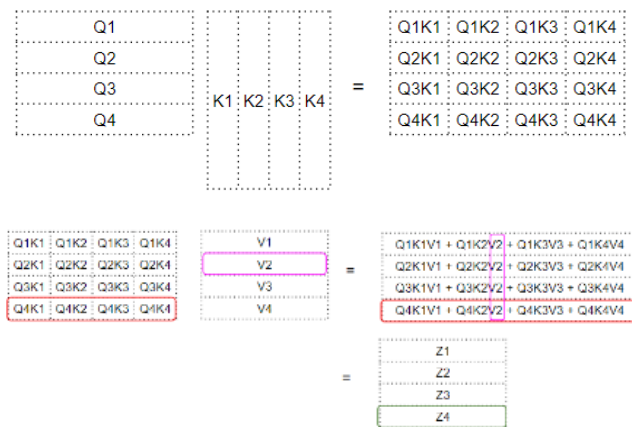
Figure 32 Matrix operations to determine attention scores.
