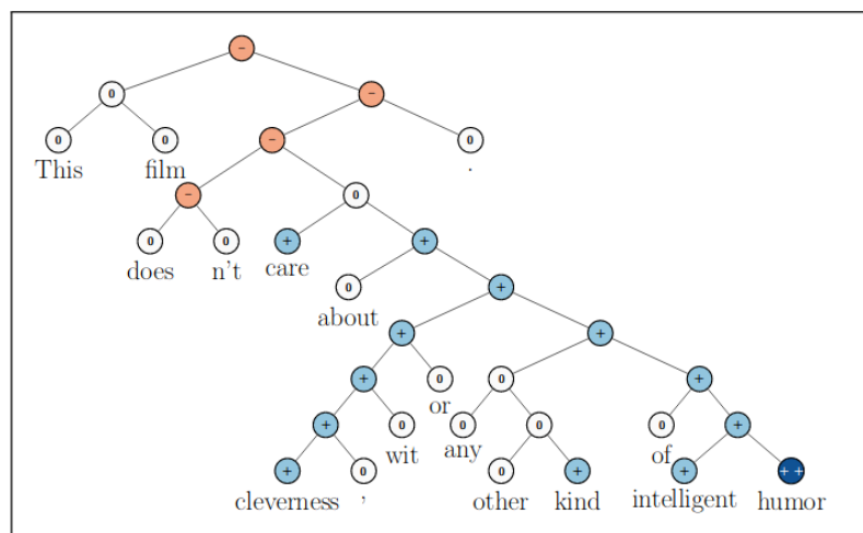
Figure 2 Fine-Grained Classification methodology of the recursive neural tensor network proposed by Socher et al. (2013).
