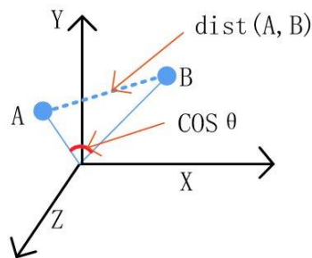
Figure 10 Cosine Similarity.
