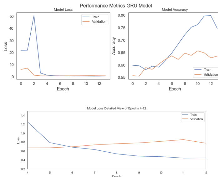
Figure 21 Training Profile of Optimal GRU model.
