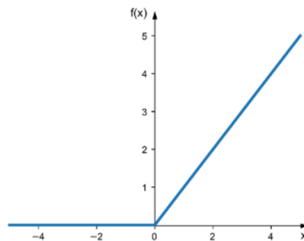
Figure 26 ReLU activation function graph.
