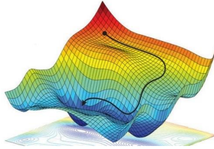
Figure 23 3D visualisation of complex loss landscape. The model must be capable of escaping saddle points and local minima to reach the global optimal solution.
