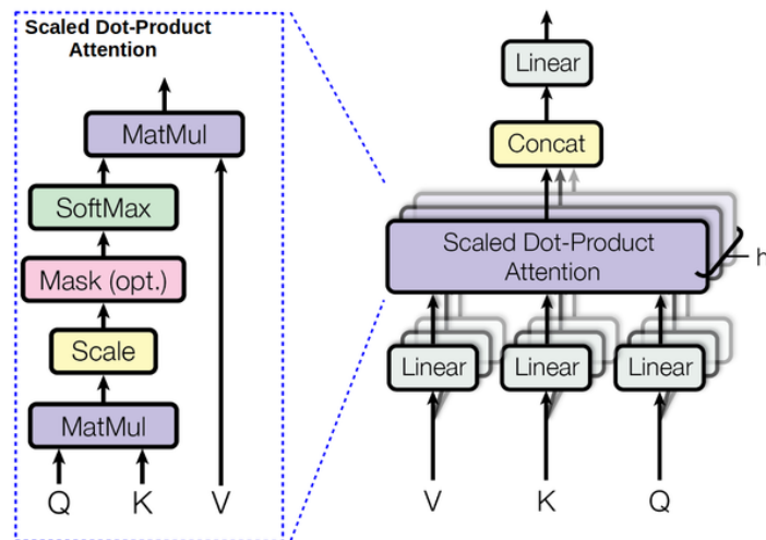
Figure 32 Matrix operations to determine attention scores.
