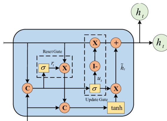
Figure 31 GRU unit architecture.
