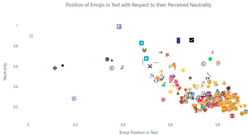
Figure 8 Degree of Neutrality (Neutral Sentiment Score) against average position of emoji in text. Emojis towards the end of text strings have lower neutrality; a greater degree of arousal per dimensional emotion theory, indicative that emojis towards the end of strings are more frequently used to convey tone or emotion compared to those appearing earlier in the string. This observation is consolidated by the frequency of face emojis, which are intuitively linked to tone and emotion with low neutrality scores at the end of sentences.
