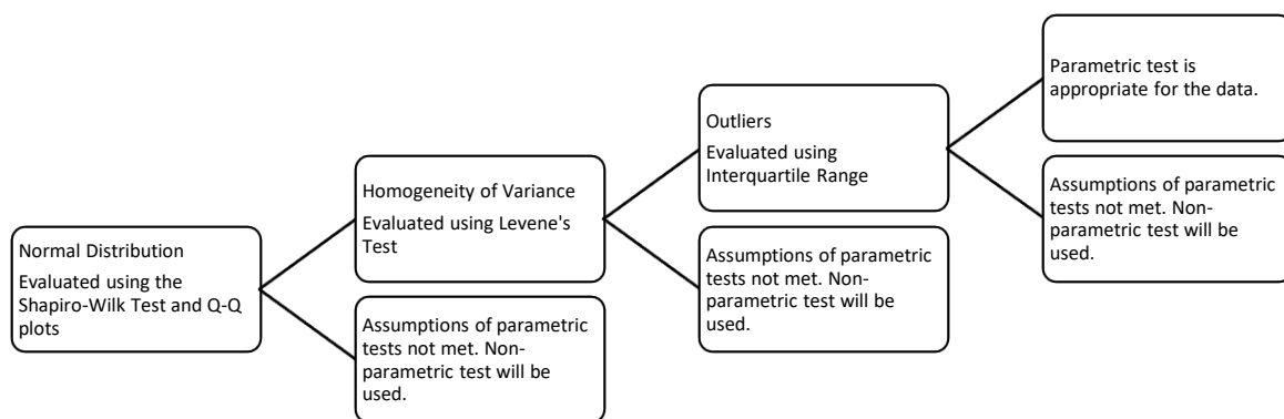
Figure 38 Process flow chart to determine if data under evaluation is parametric or non-parametric.
